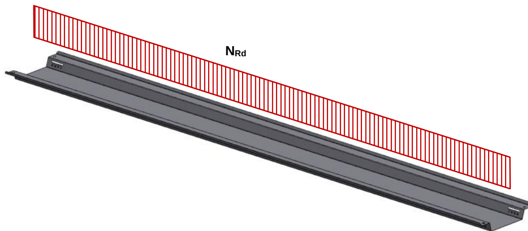
Fig. 6: Illustration of the load effect on the ballast tray MSP-FR-S-WD
