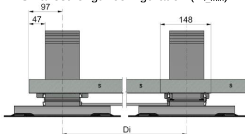
Smallest length configuration (D i_min )
