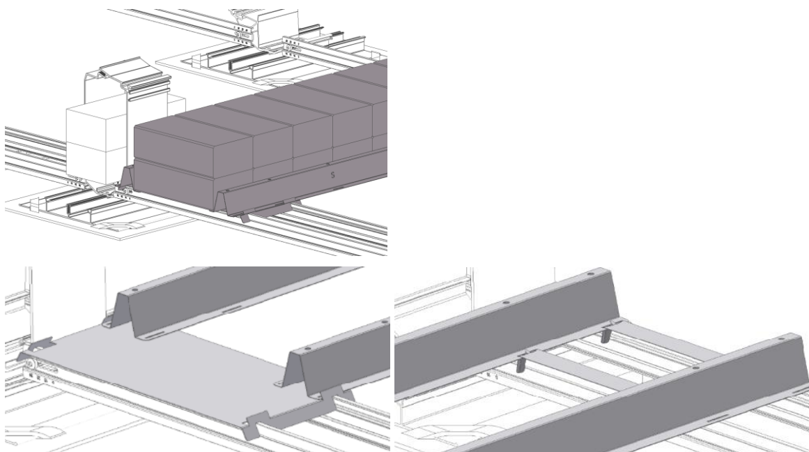
Fig. 4: Stiffening of the connection channels
