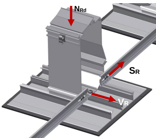
Fig. 2: Vectors of the rated resistances MSP-FR-S-SH
