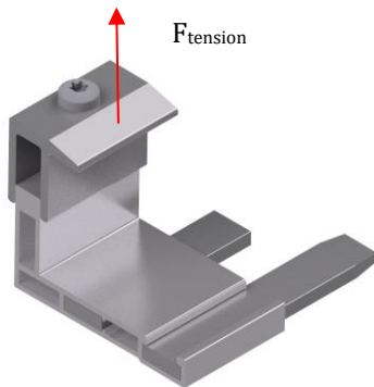
Fig. 8: Vectors of resistance of the complementary clamp low MSP-FR-LC/B
