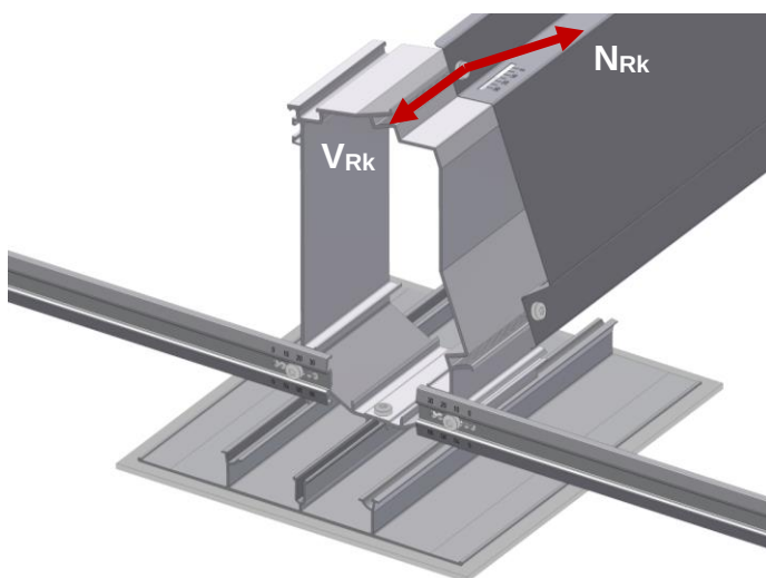
Fig. 1: Vectors of the rated resistances for the fastening of the wind deflector MSP-FR-S-WD
