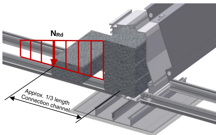
Fig. 3: Vectors of resistance of MSP-FR-EW-C
