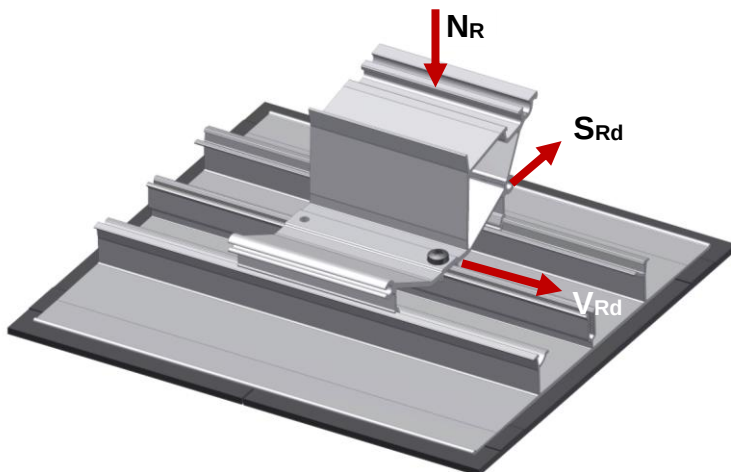
Fig. 1: Vectors of the rated resistances of MSP-FR-S-SL8/SL10
