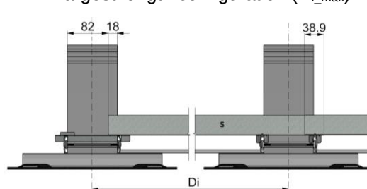
Largest length configuration (D i_max )
