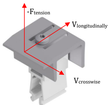
Fig. 8: Vectors of resistance of the end clamp MSP-PR-EC/B
