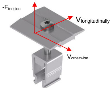
Fig. 6: Vectors of resistance of the middle clamp MSP-PR-MC/G & MSP-PR-MCB/G
