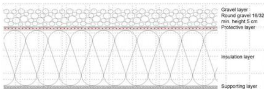
Figure 1: typical structure of a gravel roof
