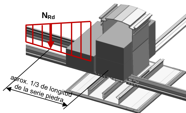
Fig.3 : Vectores de resistencia de MSP-FR-EW-C
