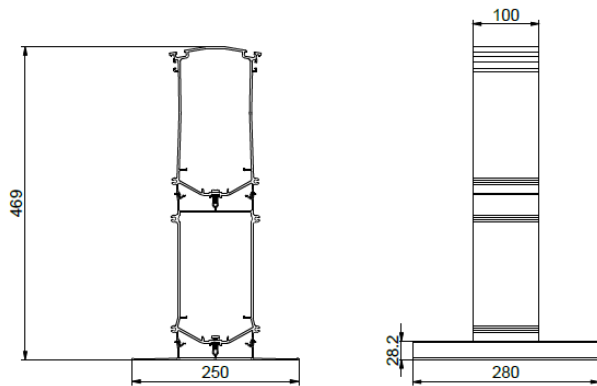
Fig. 12 : Green roof support high
