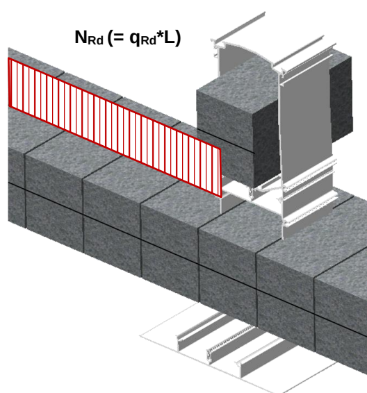
Fig. 11: Illustration of the load effect on MSP-FR-EW-C
