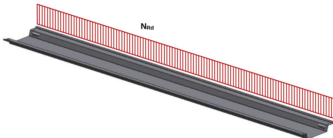
Fig. 5: MSP-FR-S-WD visualisation of the load effect
