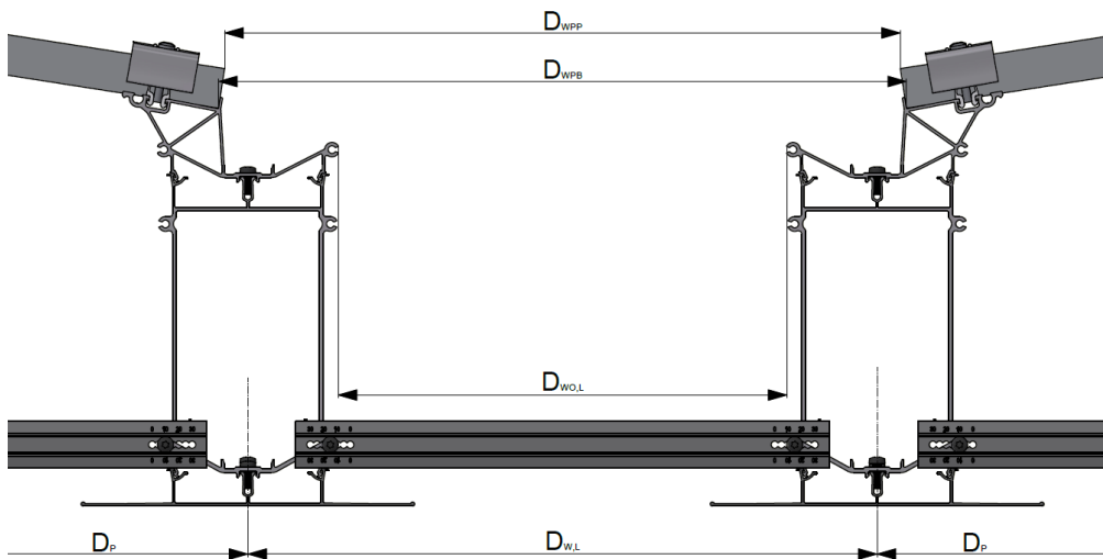
Fig. 16: Walkway on the eaves
