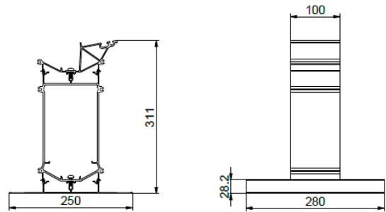
Fig. 13: Green roof support low
