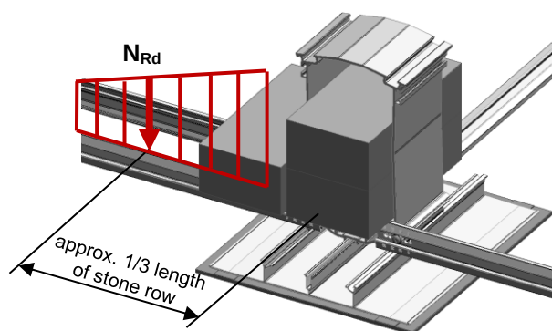
Fig.3 : Vectors of resistance vectors of MSP-FR-EW-C
