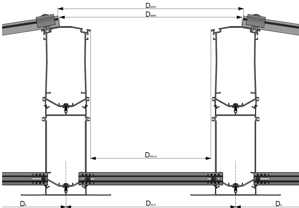
Fig. 16: Walkway on the ridge
