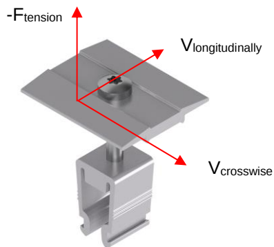
Fig. 6: Vectors of the resistance of the middle clamp
