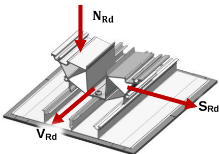
Fig.1 : Vectors of the resistance of MSP-FR-EW-SL8/SL10
