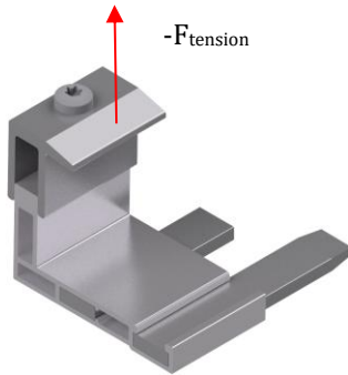
Fig. 8: Vectors of resistance of the complementary clamp low
