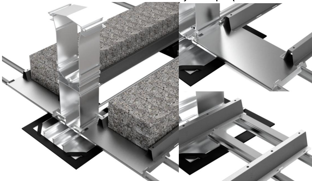
Fig.7 : Stiffening of the connection channels
