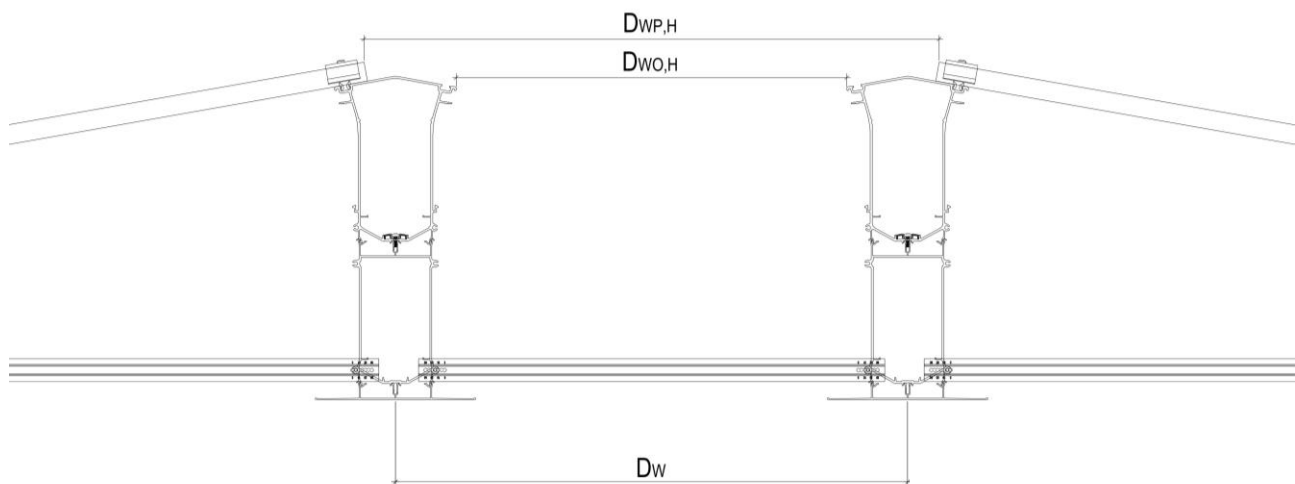
Fig.2 : Walkway at the ridge
