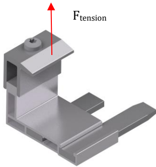
Fig.10 : Vectors of the resistance of the complementary clamp low
