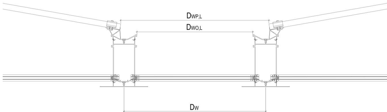
Fig. 1 : Walkway at the eaves
