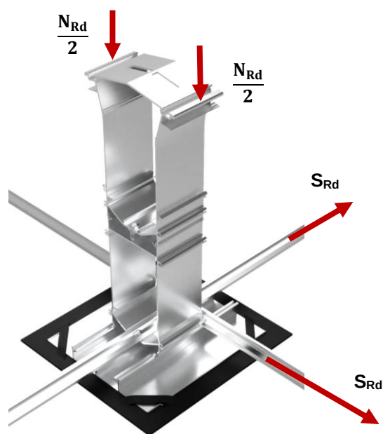
Fig.5 : Vectors of the resistances of MSP-FR-EW-SMH90
