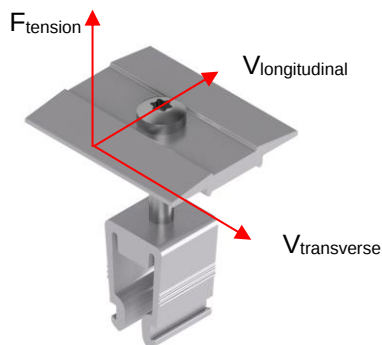
Fig.8 : Vectors of the resistances of the middle terminal
