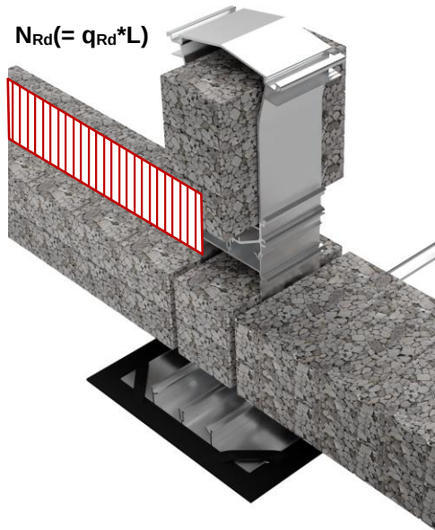
Fig.6 : Vectors of resistance of MSP-FR-EW-C and MSP-FR-BF
