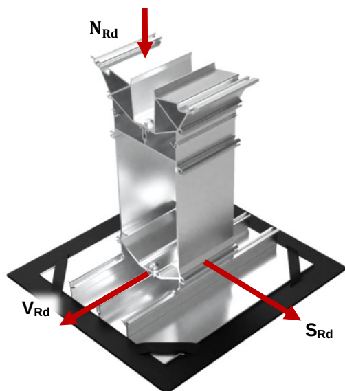
Fig. 3 : Vectors of the resistances of MSP-FR-EW-SL8/SL10
