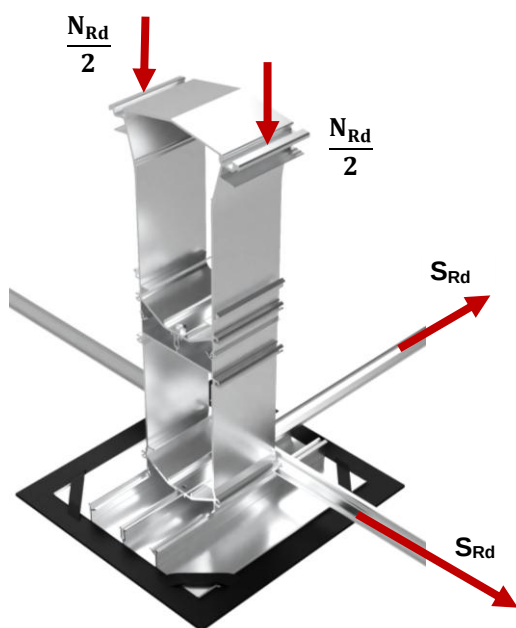
Fig.4 : Vectors of the resistances of MSP-FR-EW-SH90
