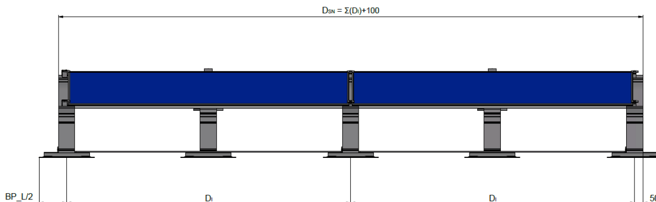
Dimensions of base profiles
