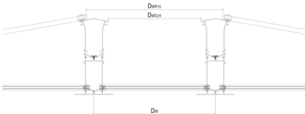
Fig.2 : Walkway at the ridge
