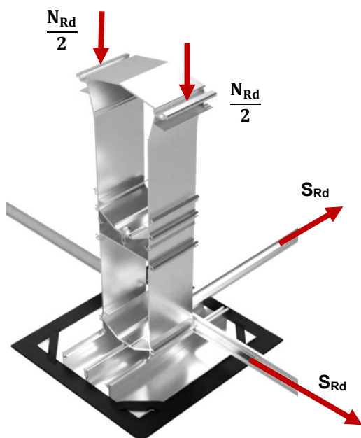
Fig.5 : Vectors of the resistances of MSP-FR-EW-SH90
