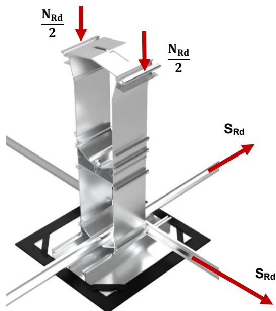
Fig.6 : Vectors of the resistances of MSP-FR-EW-SMH90
