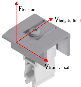
Fig.10 : Vectors of the resistance of the end clamp
