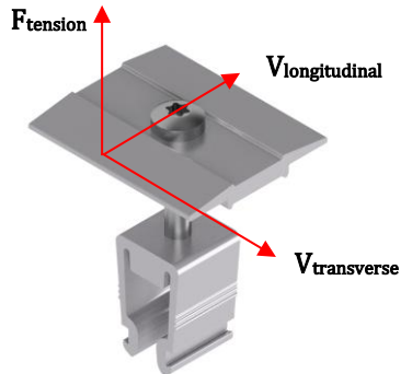
7 : Resistance vectors of the middle clamp
