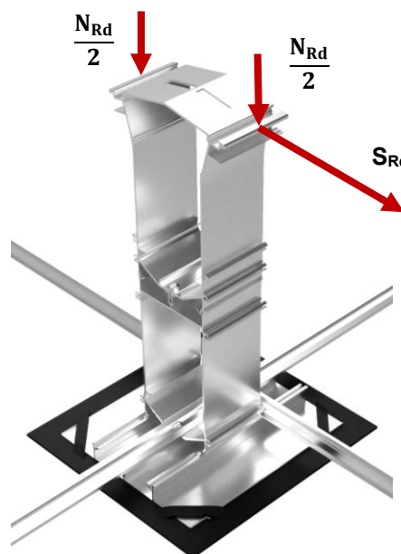
Fig.6 : Vectors of the resistances of MSP-FR-EW-SMH90
