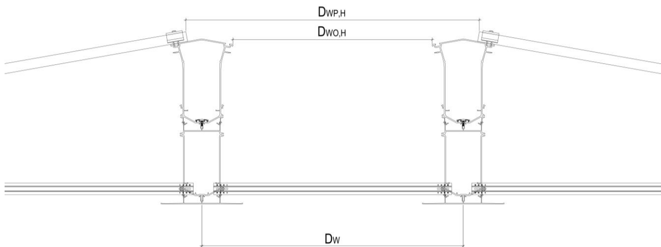
Fig.2 : Walkway at the ridge – 30 mm module
